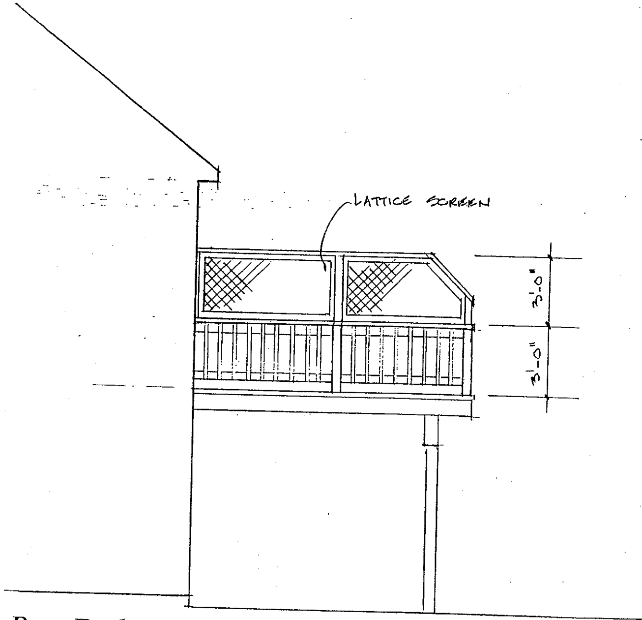
Rear Deck Privacy Screen (Type B)
