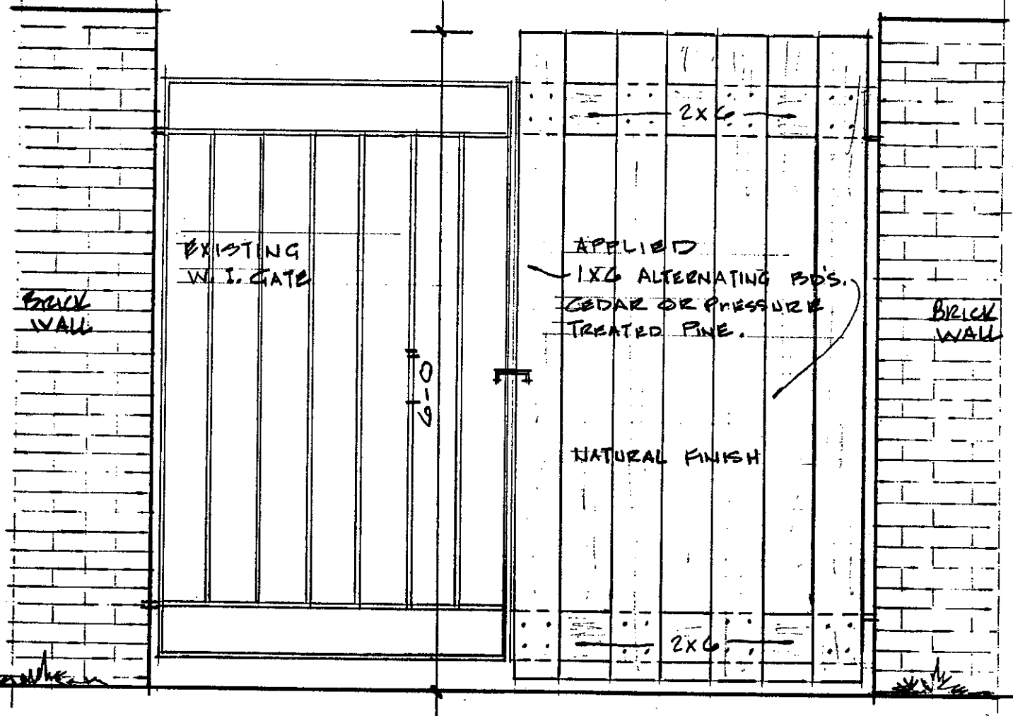
Garden Wall Iron Gate/Privacy Screen
