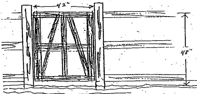
Split-rail Gate
